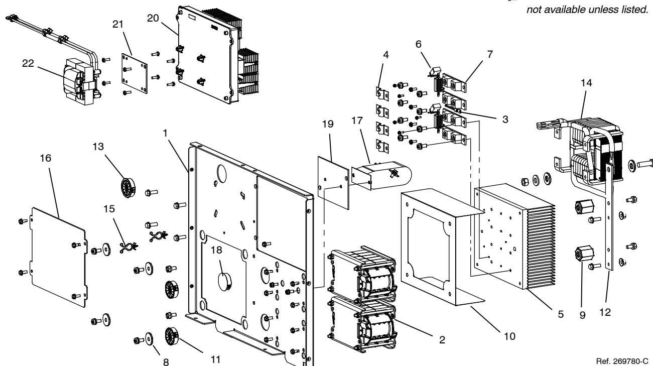
Figure 1-2. Right-Hand Windtunnel w/Components
