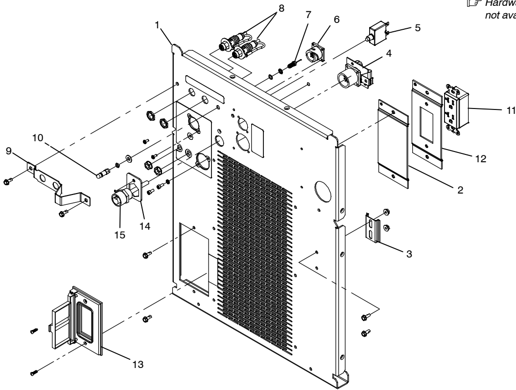
Figure 1-8. Rear Panel Assembly Eff w/Serial No. MJ360517C
