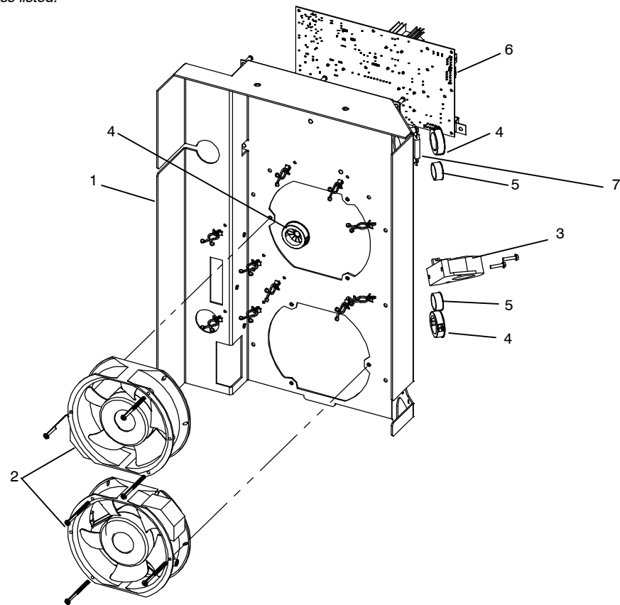
Figure 2-4. Fan Panel Assembly
