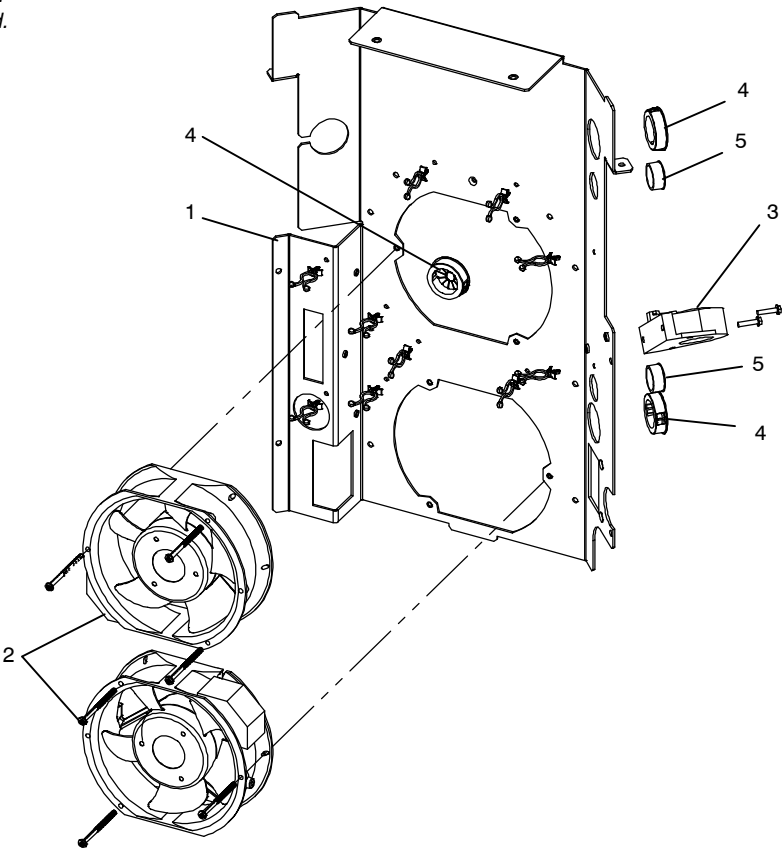
Figure 1-4. Fan Panel Assembly
