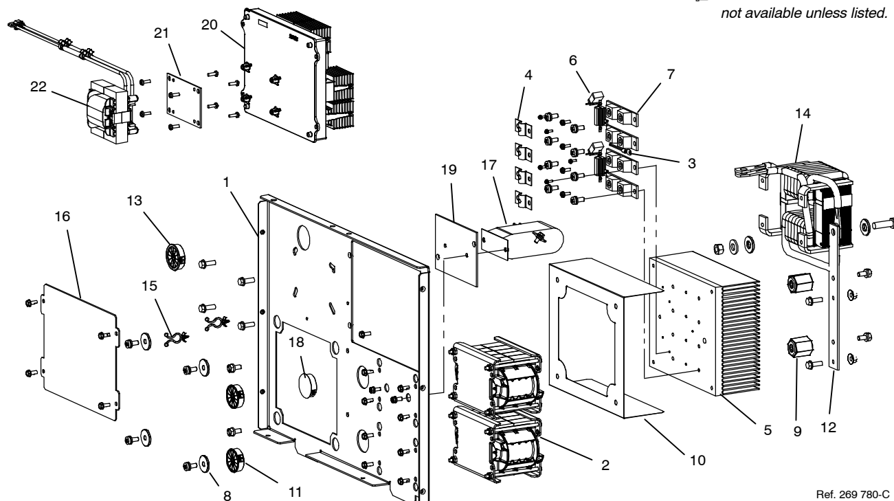
Figure 2-2. Right-Hand Windtunnel w/Components
