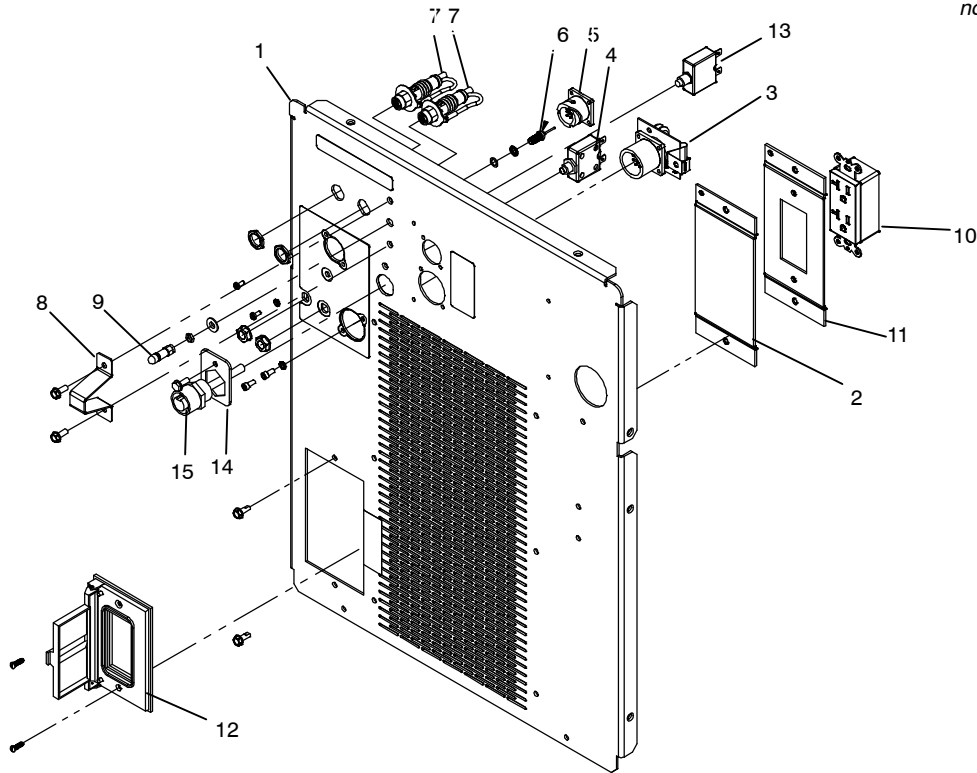
Figure 2-7. Rear Panel Assembly
