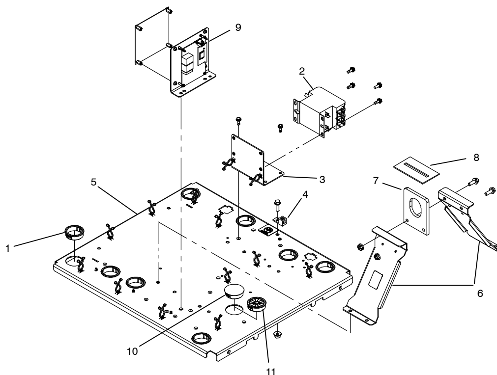
Figure 2-6. Penthouse Assembly
