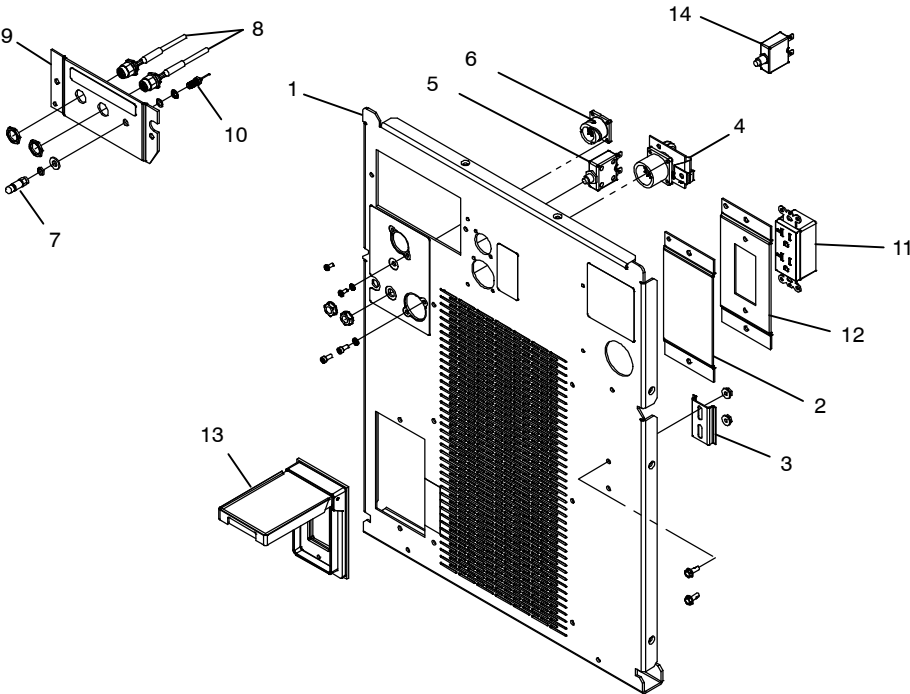
Figure 1-7. Rear Panel Assembly Prior To MJ360517C
